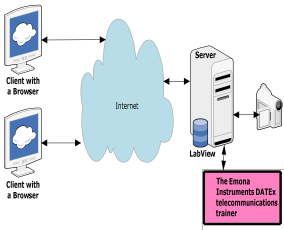
Figure 2: Remote Communications laboratory based on the DATEX-Elvis II setup
